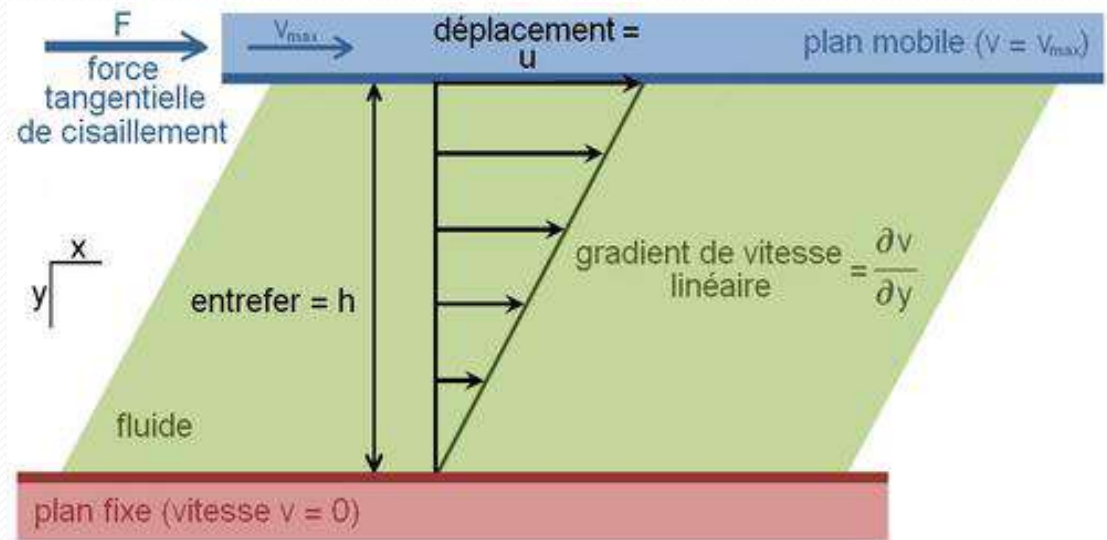
Figure I.1: Frottement visqueux
